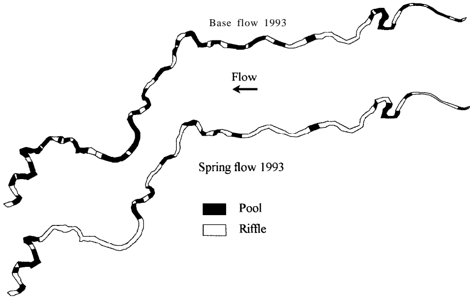
FIGURE 1.—Pool-riffle sequencing in Stony Creek during base flow and elevated spring flow conditions. The mapped section is 870 m in length. Note that the stream width was held constant between periods for visual purposes.
